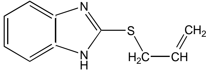
2-(2-Propenylthio)-1-H- benzimidazole (PTHB)
