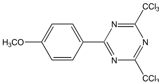
2-(4'-Methoxyphenyl)-4,6-bis(trichloromethyl)-1,3,5-triazine
